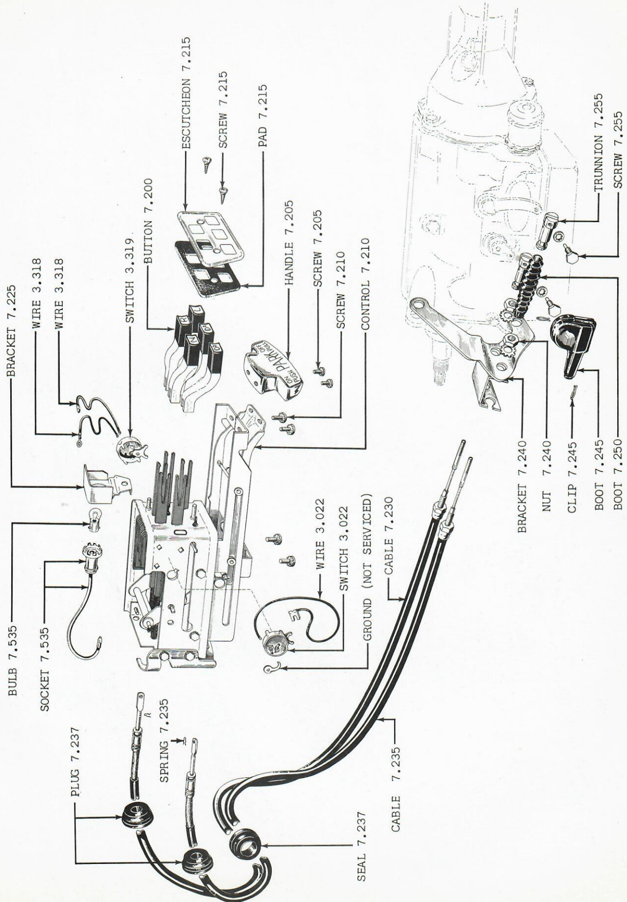
GROUP 7 - FIG. 4 - PUSH BUTTON SHIFTING 10-20-80 (WAT)
