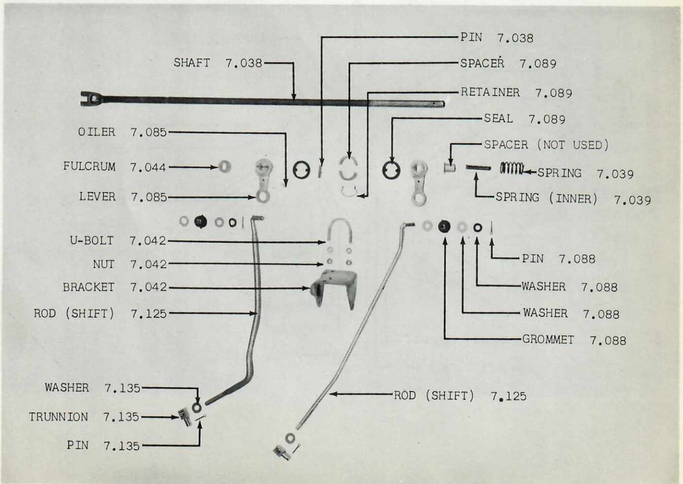
GROUP 7 - FIG. 2 - GEAR SHIFT LINKAGE (LOWER) 01 (LAT)
